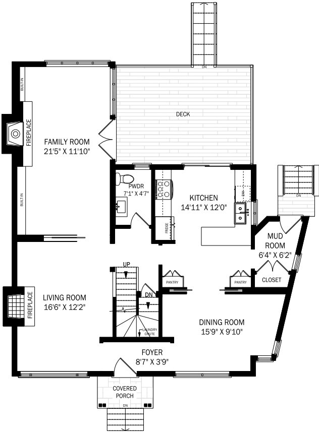
CEILING HEIGHT 8'3" MAIN FLOOR - 1089 SQUARE FEET
